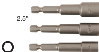
70490 3 pc. Hex Inch Nut Setter Set Permanent industrial magnet. 65mm OAL Hex Inch Nut Setters.
