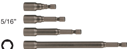
704 Nut Setters Standard. 5/16" Hex Inch Permanent industrial magnet.
